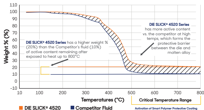
TGA Curve Comparison of DIE SLICK® 4520 Series vs. Competitive Product
